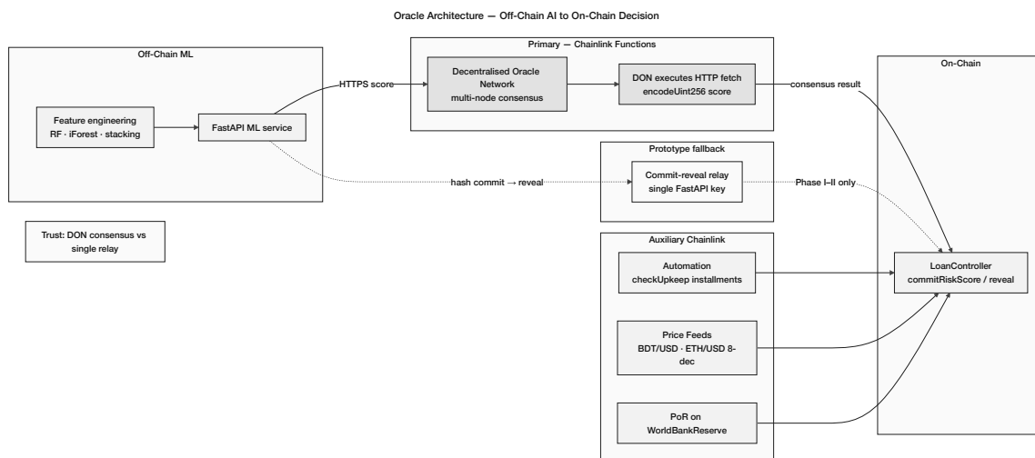
Figure 3.5: Oracle architecture: Chainlink Functions DON as the primary path for ML risk-score commitment to LoanController; commit-reveal FastAPI relay as prototype fallback; Chainlink Automation, Price Feeds, and Proof of Reserve as auxiliary oracle services.
