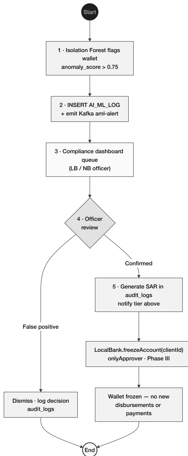
Figure 3.23: SAR activity flow: Isolation Forest flag → AI_ML_LOG → Kafka aml-alert → compliance officer review → optional freezeAccount.
