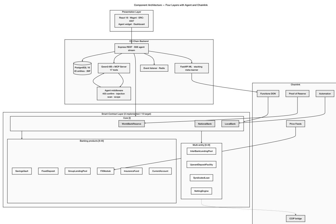
Figure 3.3: Component diagram showing interactions between the presentation layer, smart contract layer, off-chain backend services, and external systems.
