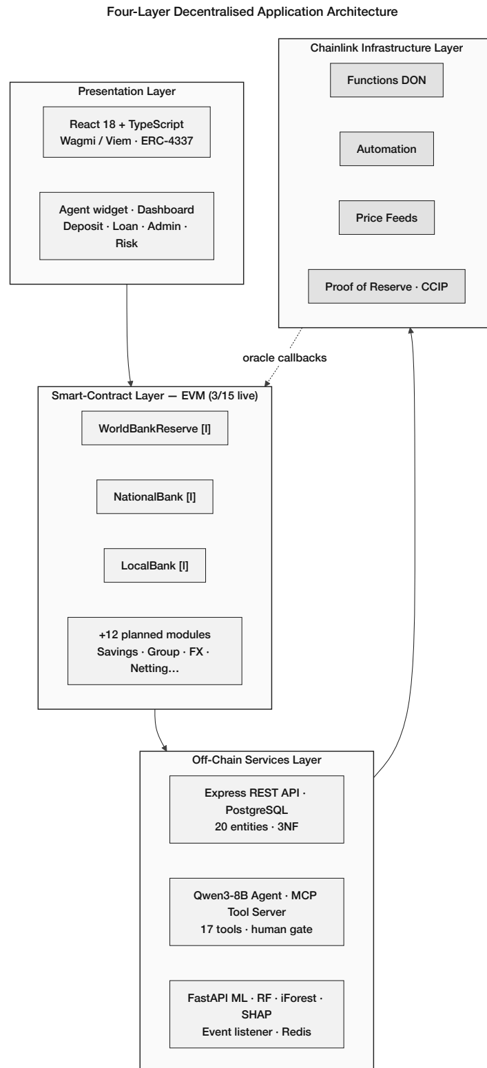
Figure 3.2: Four-layer decentralized application architecture: presentation (React 18, TypeScript, Wagmi/Viem), smart-contract layer on the EVM (World Bank Reserve, National Bank, Local Bank), off-chain services layer (Express REST API, PostgreSQL, AI Agent engine (Qwen3-8B + MCP Tool Server), Chainlink oracle integration, event listener, Redis), and Chainlink infrastructure layer (Chainlink Functions, Automation, Price Feeds, Proof of Reserve).
